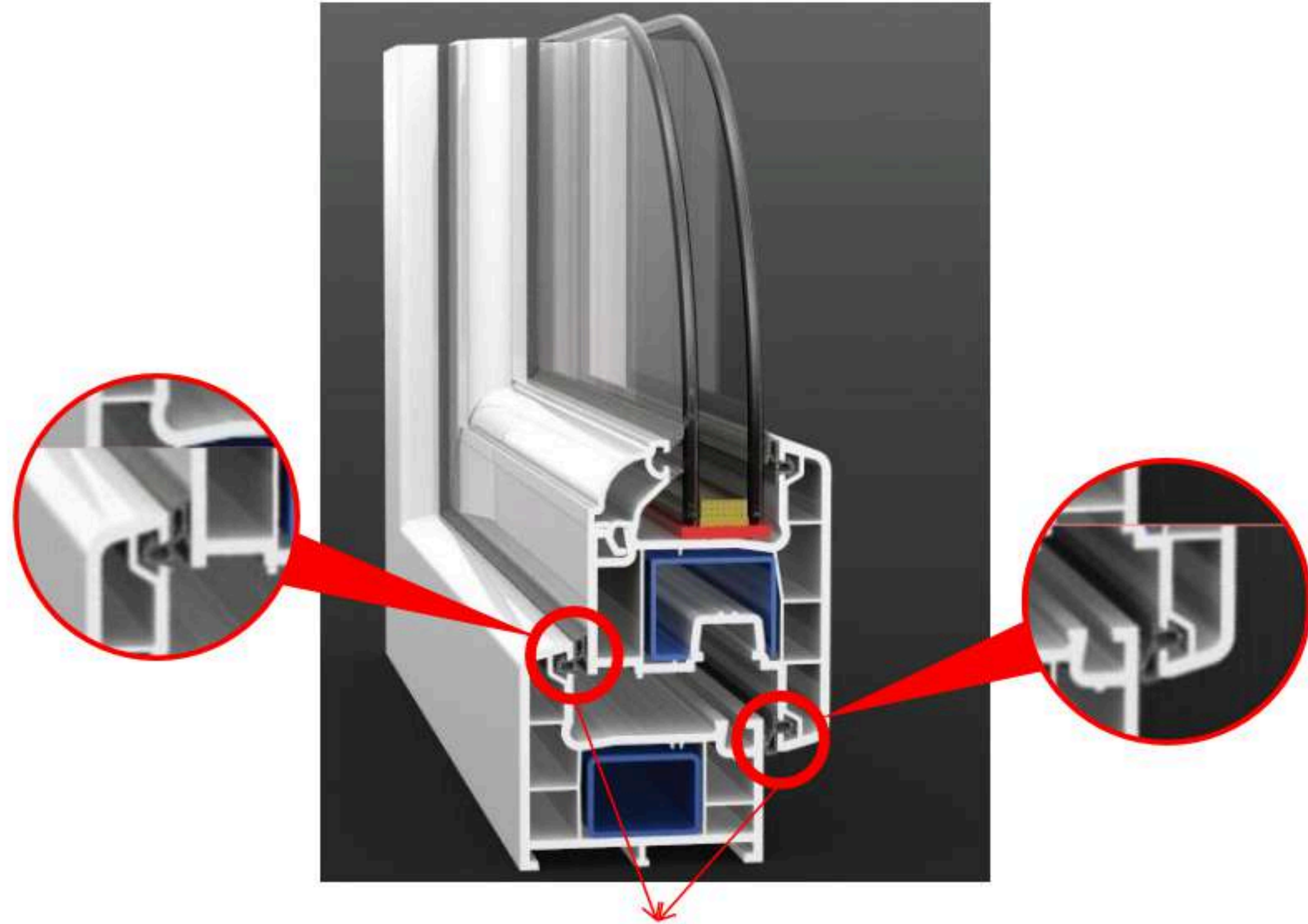
Double layer of sealing
